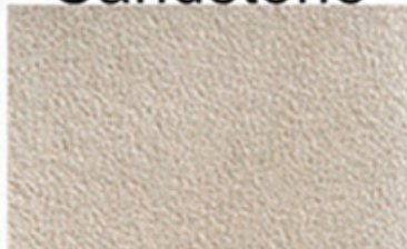
Sandstone
