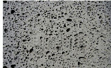
Volcanic rocks
