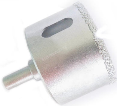
Vacuum brazed diamond core bits with round shank
