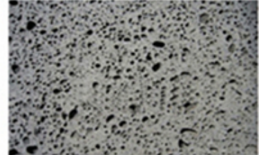
Volcanic rocks
