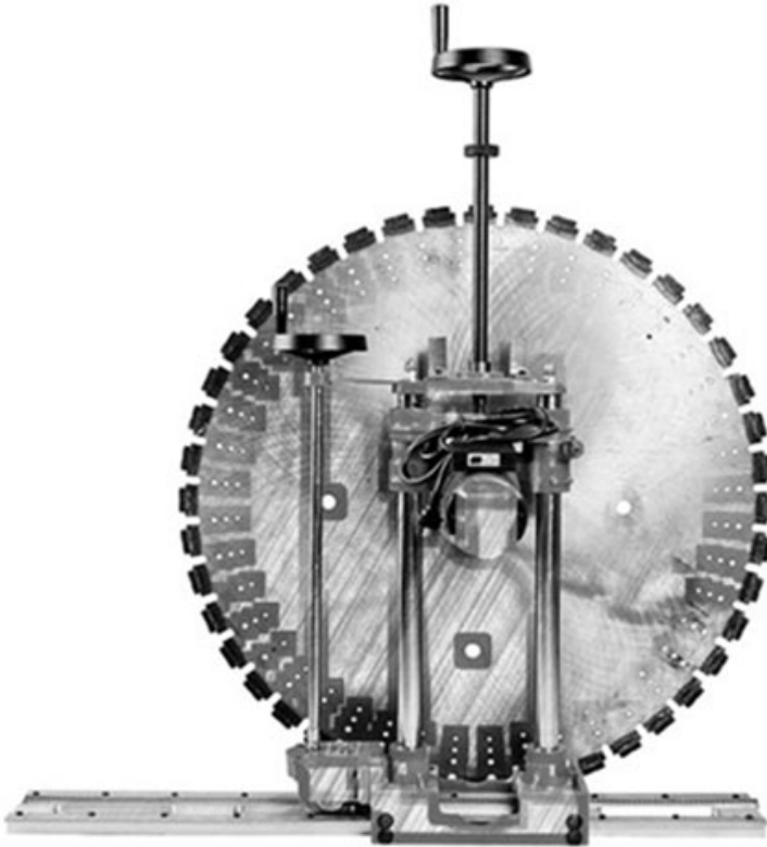
Wall Cutting Machine
