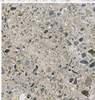
Quartz
