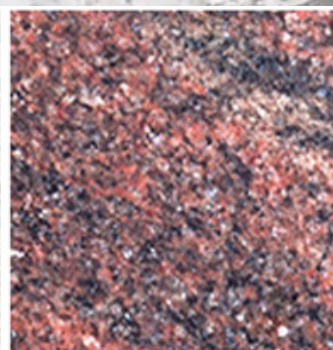
Granite
