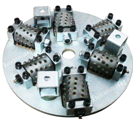
300MM Floor Bush Hammer Plate
