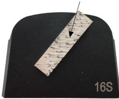
Lavina Tools With Single Diamond Grinding Segment
