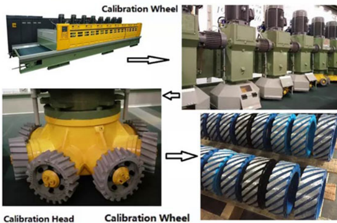
Calibration Head
