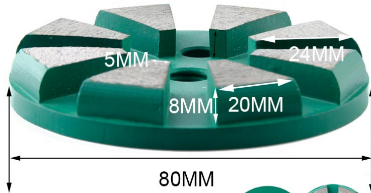
Single Arc Segments Concrete Grinding Disc
