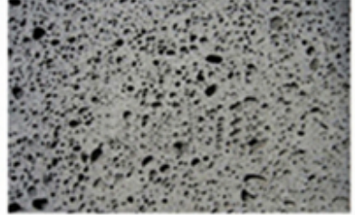
Volcanic rocks
