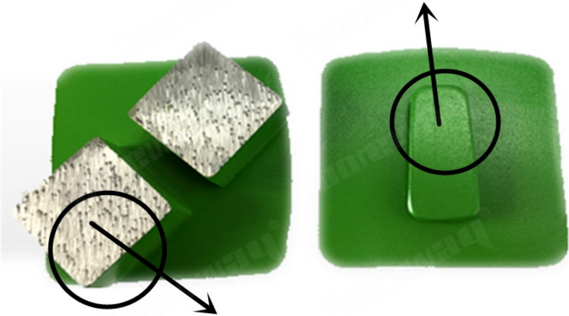
20*20*10mm*2T Double Square Segments
