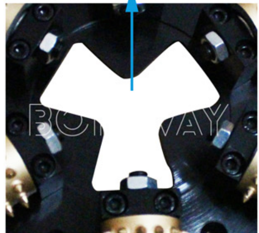
HTC Quick Change Connector
