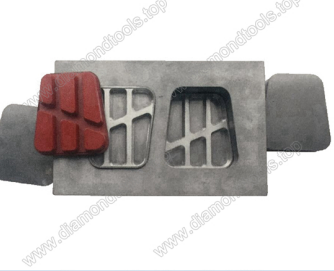
Mould for diamond floor grinding blocks
