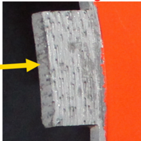
Diamond segment
