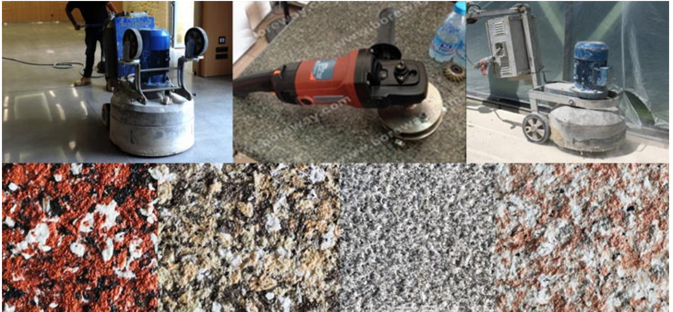
45 Pins Carbide Alloy Bush Hammer Roller Application Disc:
