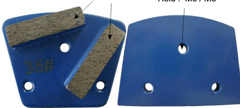
Segment Sizes : 40*10*10*2T (mm) Hold : M6 / M8
