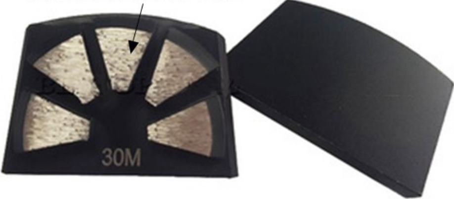
Lavina Diamond Floor Grinding Disc Segment Shape:5T*Fan Shape Segment
