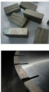
Diamond saw blade welding
