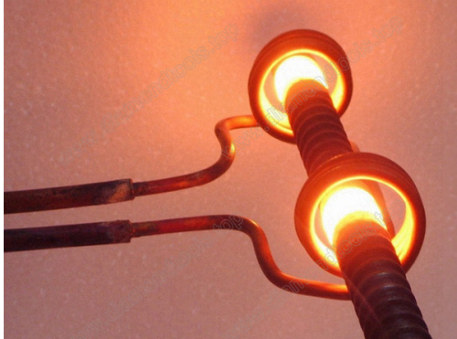
Multi-site welding
