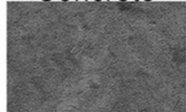
Volcanic rocks
