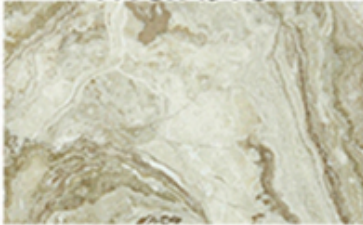
Sandstone
