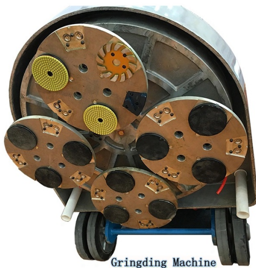
Grinding Machine
