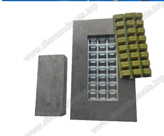
Mould for diamond floor grinding blocks
