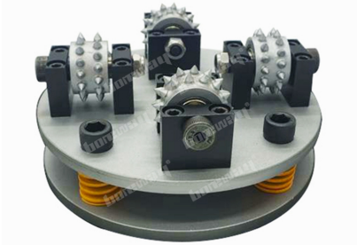
8 Zoll Bush Hammer Wheel
