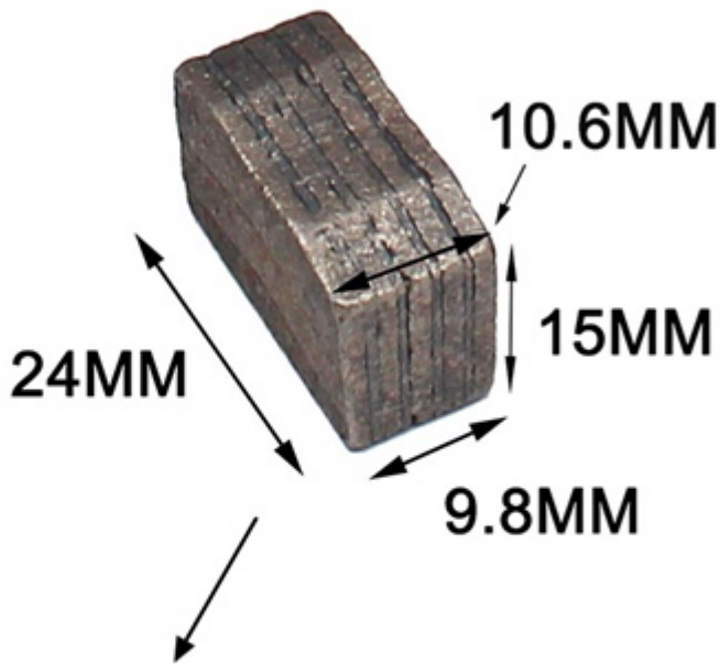
M Shape Multi Layer Structure, Good debris removal and better cooling
