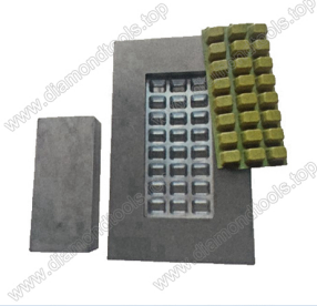
Boreway Machinery Co., Ltd. www.diamondtools.top www.boreway.com Mould for diamond floor grinding blocks
