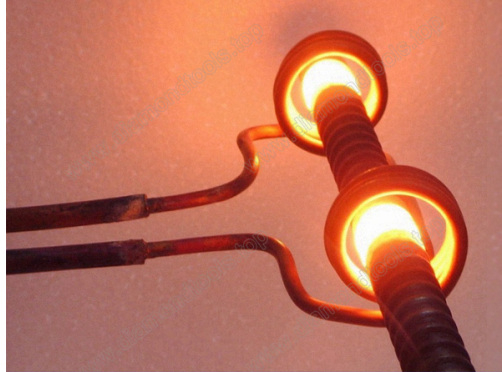
Multi-site welding
