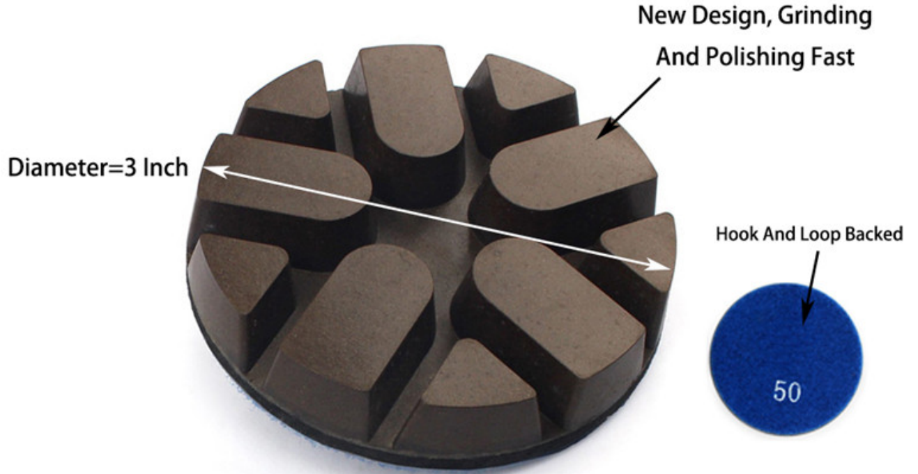
Grits 50# To 3000# Diamond Concrete Floor Grinding Polishing Discs
