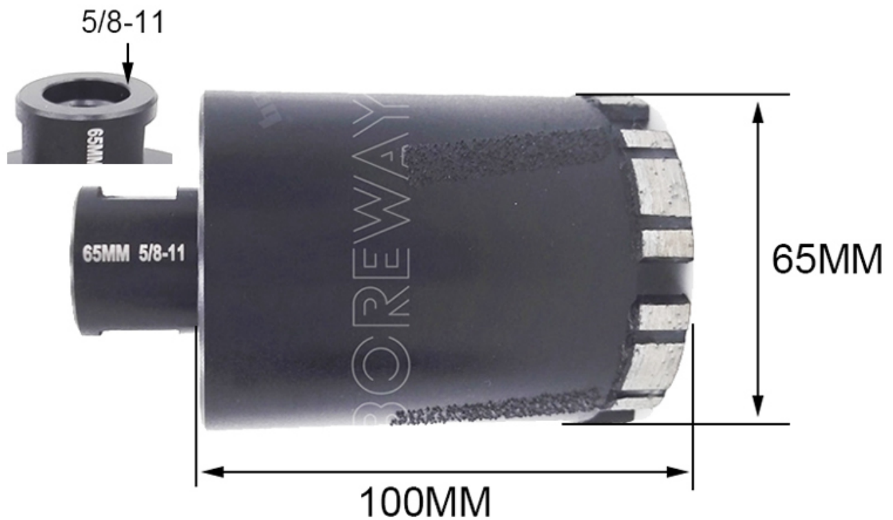
Ripple Segment
